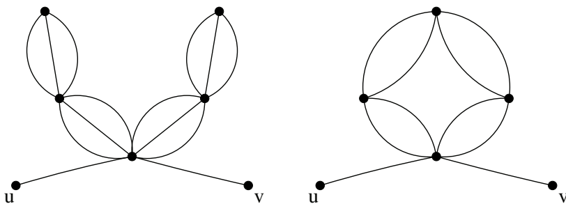
FIG. 8.1. The gadget templates T(1, 3, 2) and T(2, 2, 1) .
